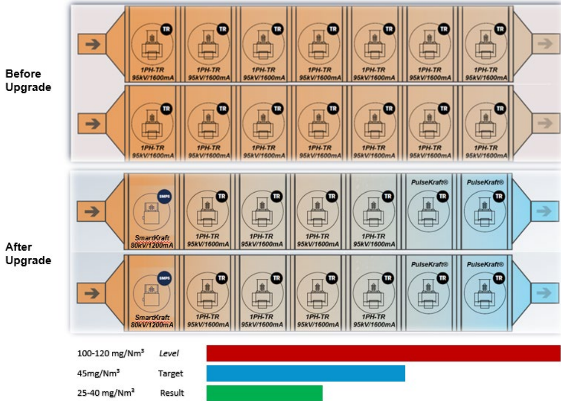
Figure 9: Power supply setup before and after upgrade
