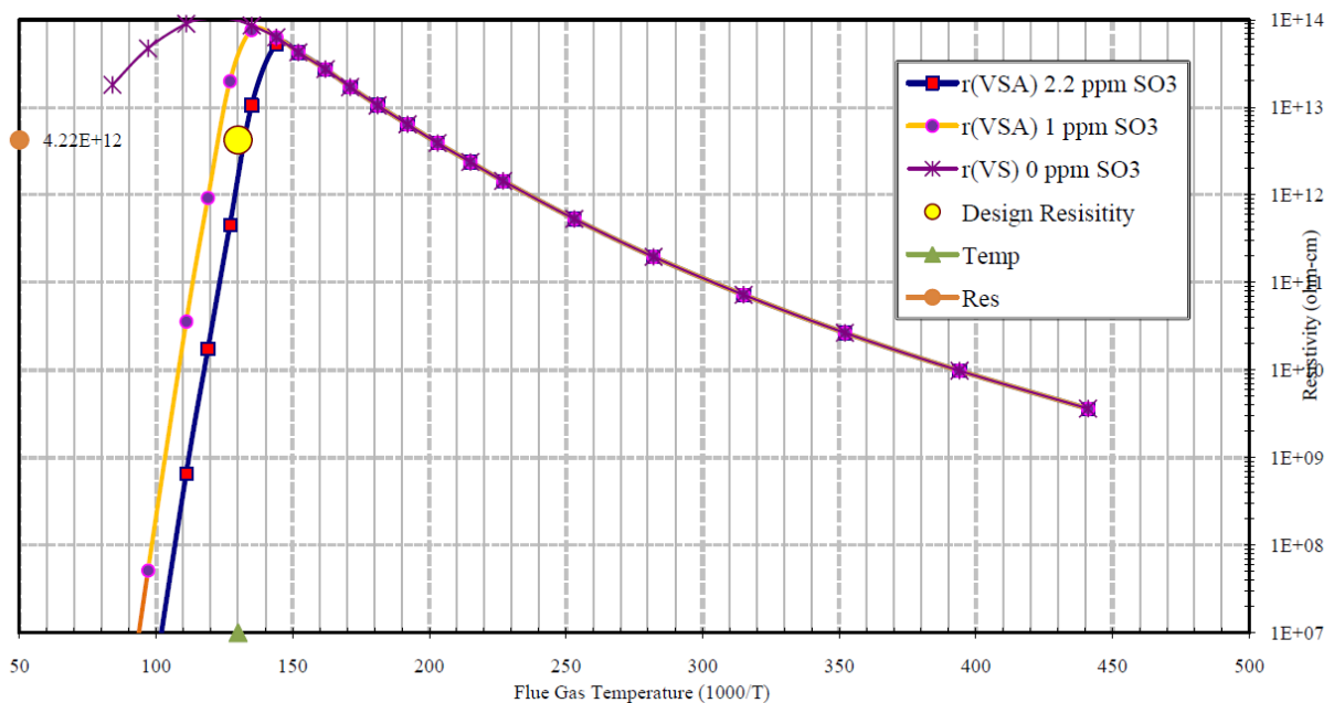
Figure 1: Fly Ash resistivity. ( 1 \times 10^{13} < \text{actual fly Ash Resistivity} < 1 \times 10^{14} \Omega\text{-cm} )
